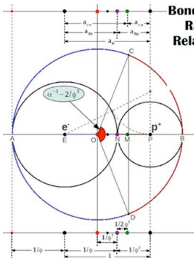
Figure 1: The Bohr radius EP = a_B of the hydrogen atom is divided into Golden sections EN = a_{Be} and NP = a_{Bp} at the point of electrical neutrality N , as the auxiliary right angle triangle makes clear. The magnetic center is located at point M , at a distance a_B/2\varphi^3 from the electrical neutrality point towards the proton. The circumference of the outer circle is also divided into two golden arcs CAD and CBD by means of the Golden angle. Note that each arc length equals the perimeter of the inner circumferences. The shorter arc is closely related to the Fine Structure constant, whose value is very near the Golden Angle shown in red. In addition, the chord CD intersects the horizontal very near the magnetic center M .
