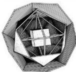
Figure 2 A WORKING MODEL OF THE NUCLEUS
