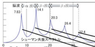
Schumann Resonance harmonics predicted by equation
